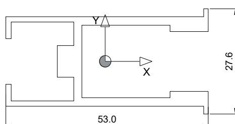
DC1057 Hoja horizontal Minimal
