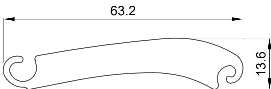
FI-5592 LAMA
