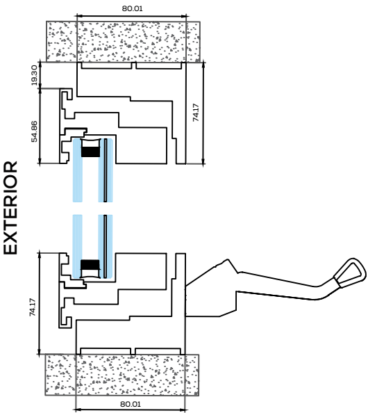
Corte Vertical
